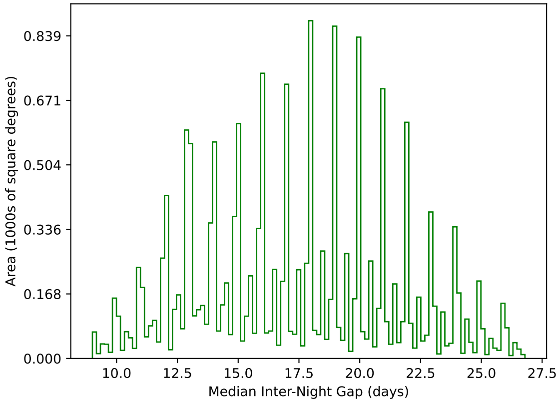
weather_cloudso18v3.4_10yrs WFD g band: Median Inter-Night Gap
