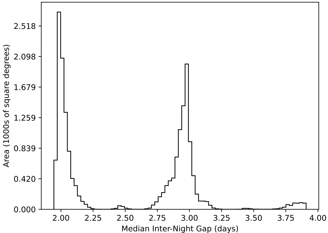
weather_cloudso18v3.4_10yrs WFD all bands: Median Inter-Night Gap
