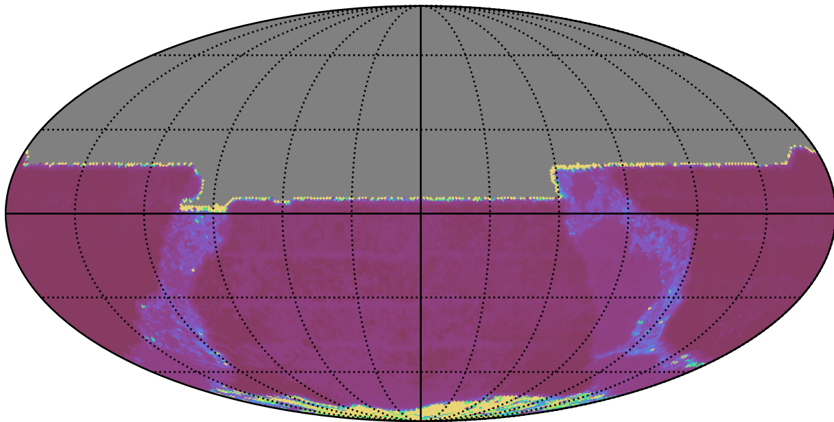
weather_cloudso18v3.4_10yrs All sky y band: Median Inter-Night Gap
