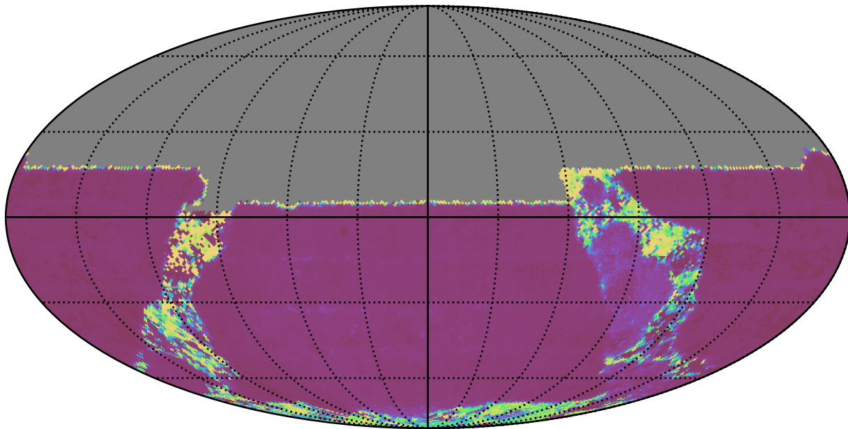
weather_cloudso18v3.4_10yrs All sky u band: Median Inter-Night Gap
