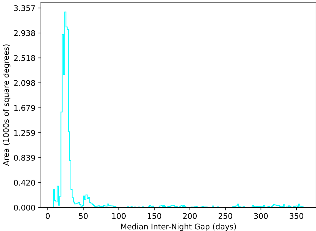
weather_cloudso18v3.4_10yrs All sky u band: Median Inter-Night Gap
