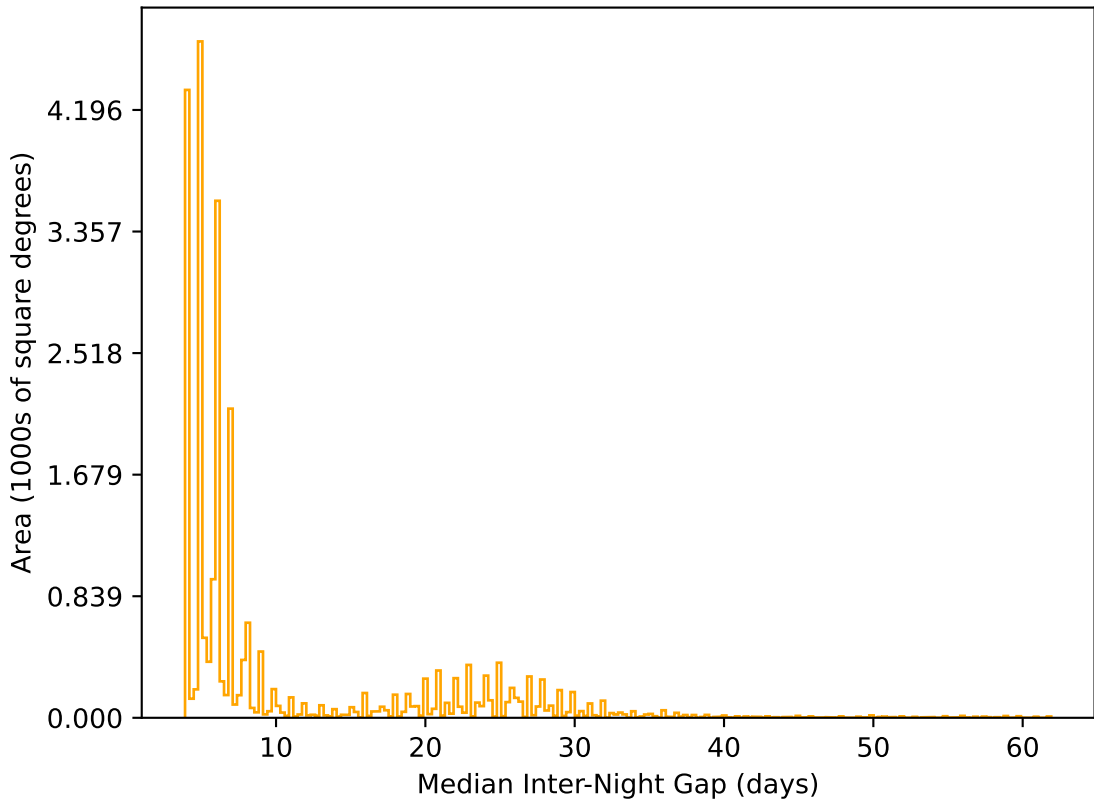
weather_cloudso18v3.4_10yrs All sky r band: Median Inter-Night Gap
