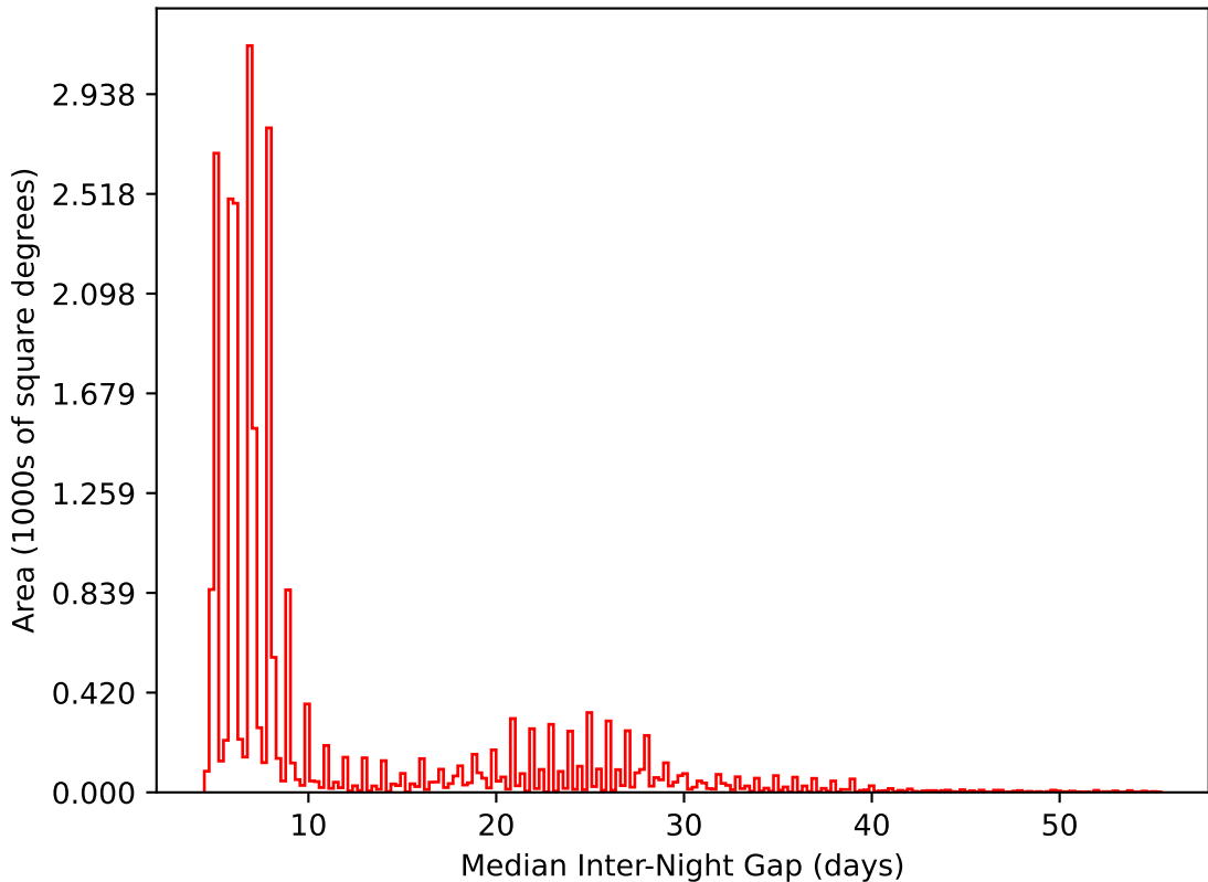
weather_cloudso18v3.4_10yrs All sky i band: Median Inter-Night Gap
