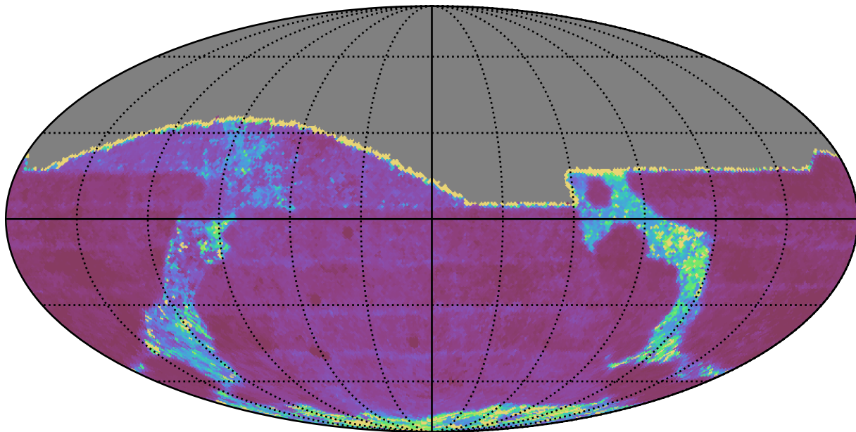
weather_cloudso18v3.4_10yrs All sky g band: Median Inter-Night Gap
