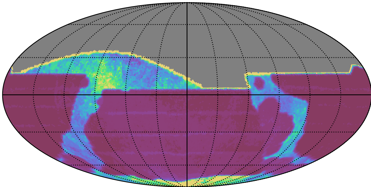
weather_cloudso18v3.4_10yrs All sky all bands: Median Inter-Night Gap
