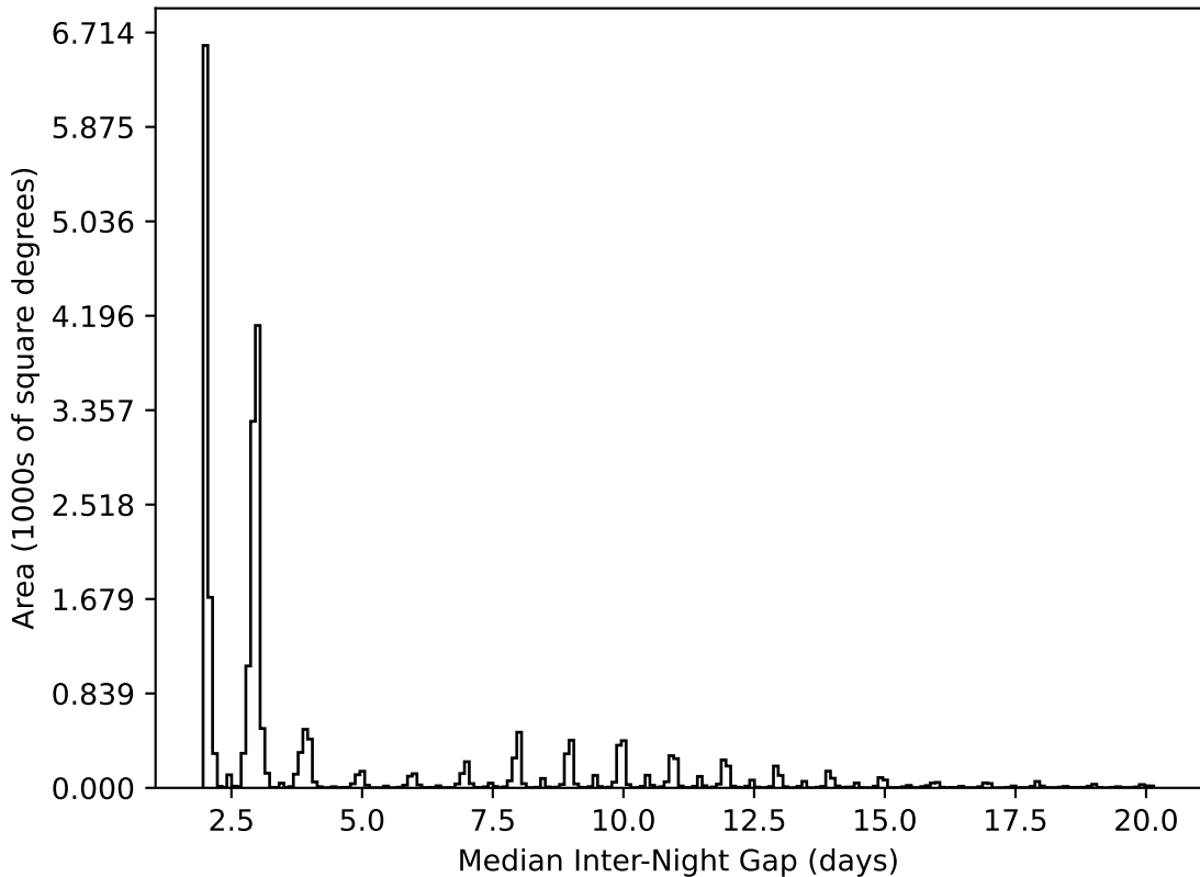
weather_cloudso18v3.4_10yrs All sky all bands: Median Inter-Night Gap
