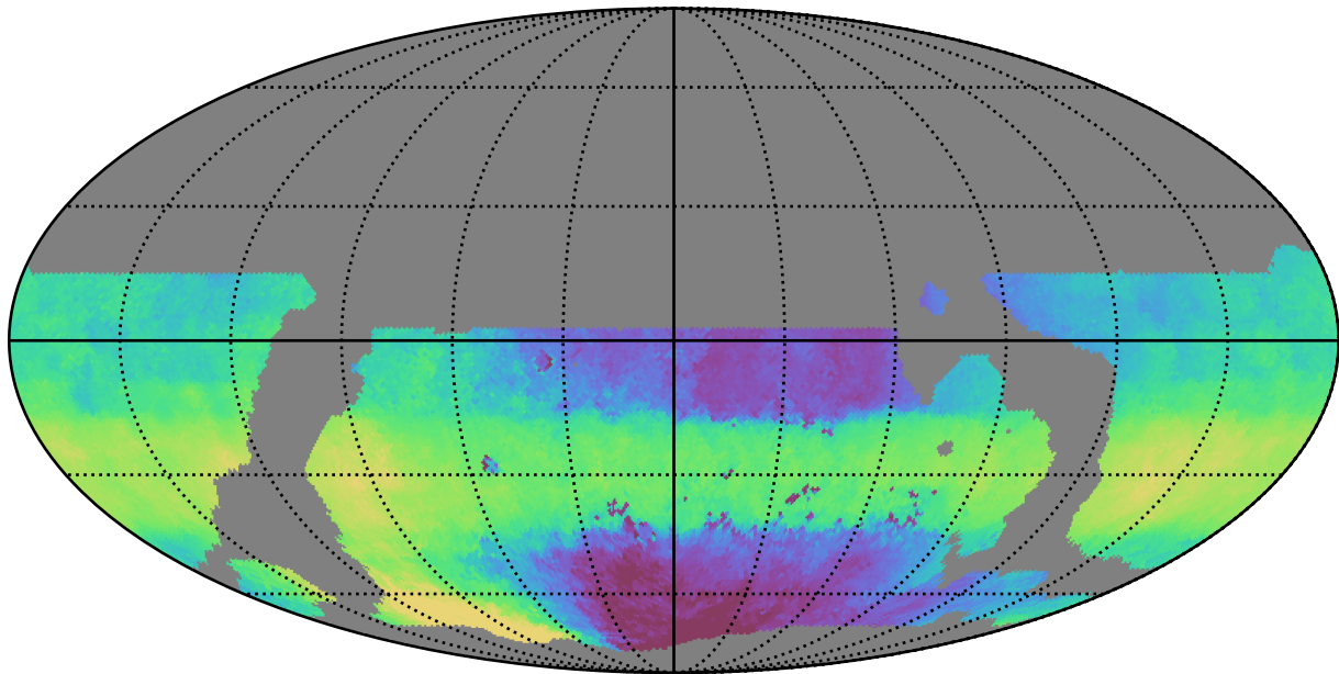
weather_cloudso18v3.4_10yrs WFD z band: Median HA
