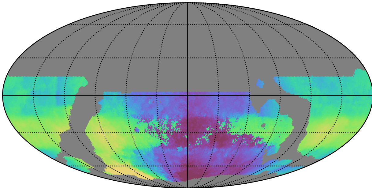
weather_cloudso18v3.4_10yrs WFD r band: Median HA
