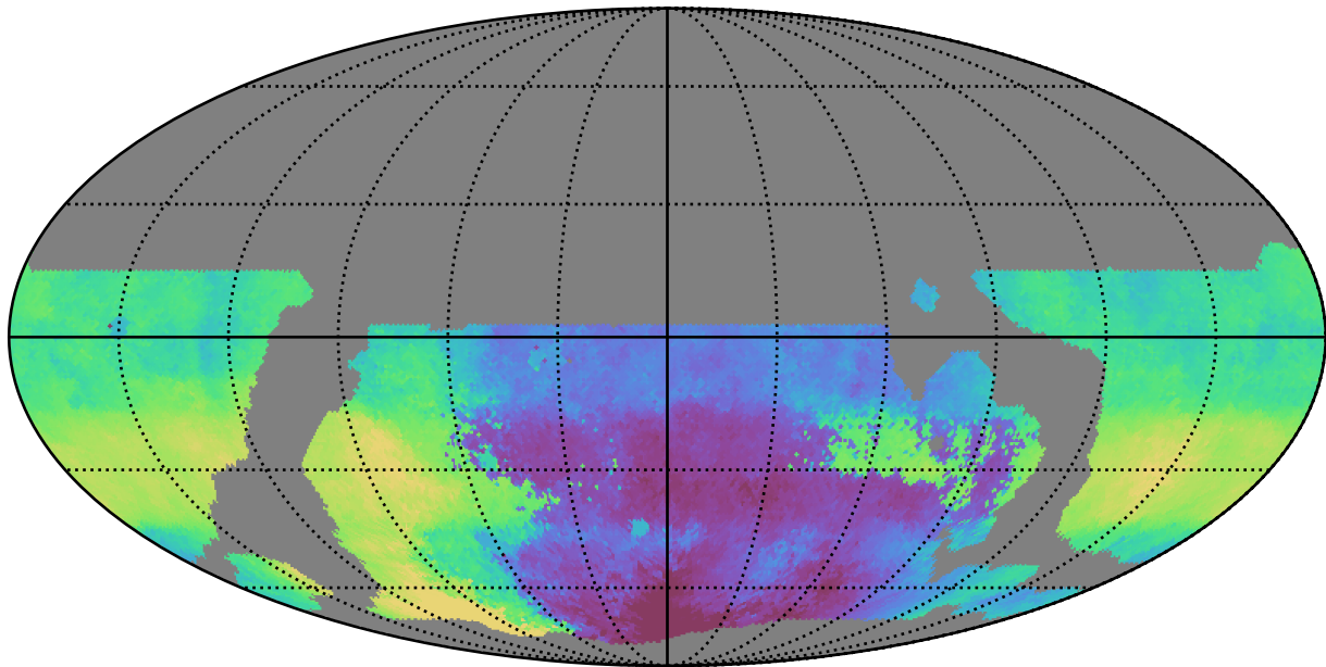
weather_cloudso18v3.4_10yrs WFD g band: Median HA
