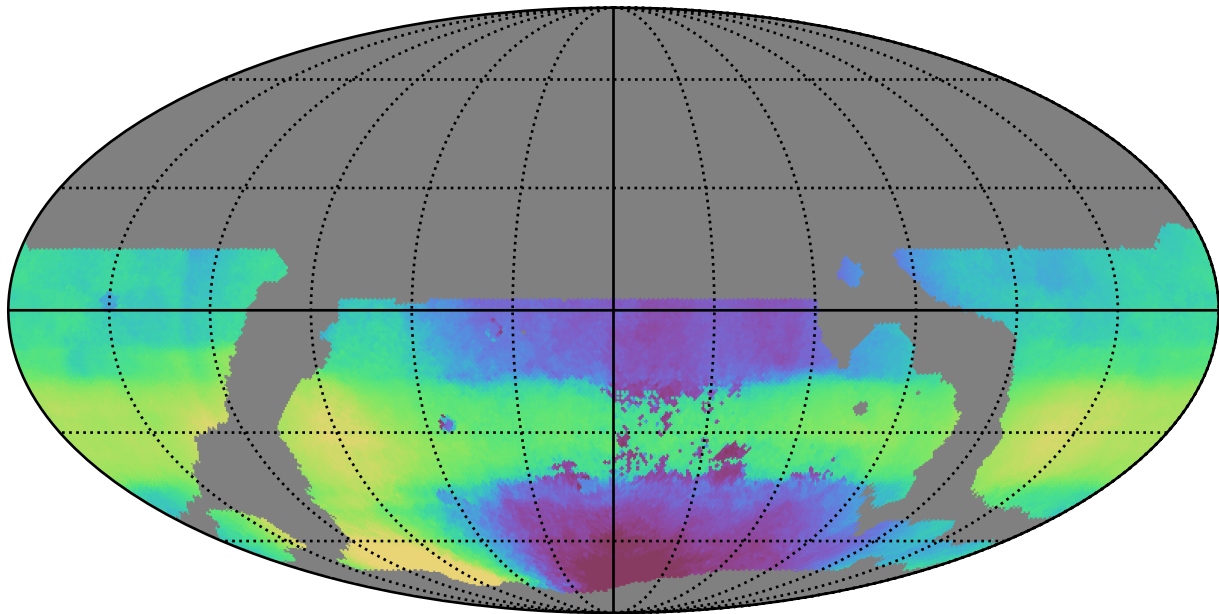
weather_cloudso18v3.4_10yrs WFD all bands: Median HA
