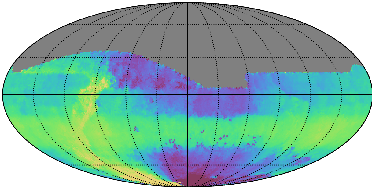
weather_cloudso18v3.4_10yrs All sky z band: Median HA
