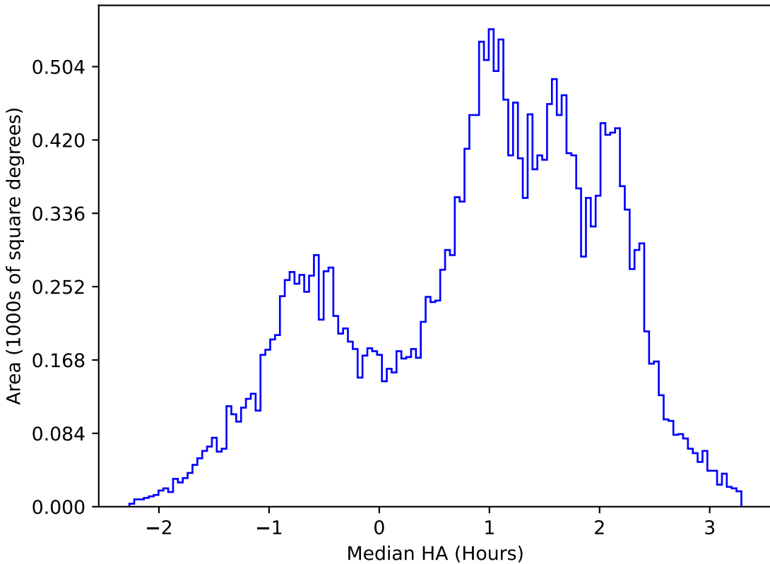
weather_cloudso18v3.4_10yrs All sky z band: Median HA
