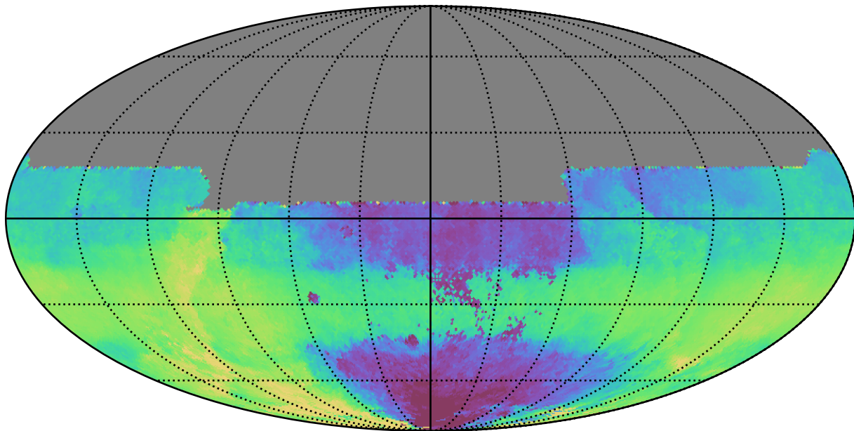
weather_cloudso18v3.4_10yrs All sky y band: Median HA
