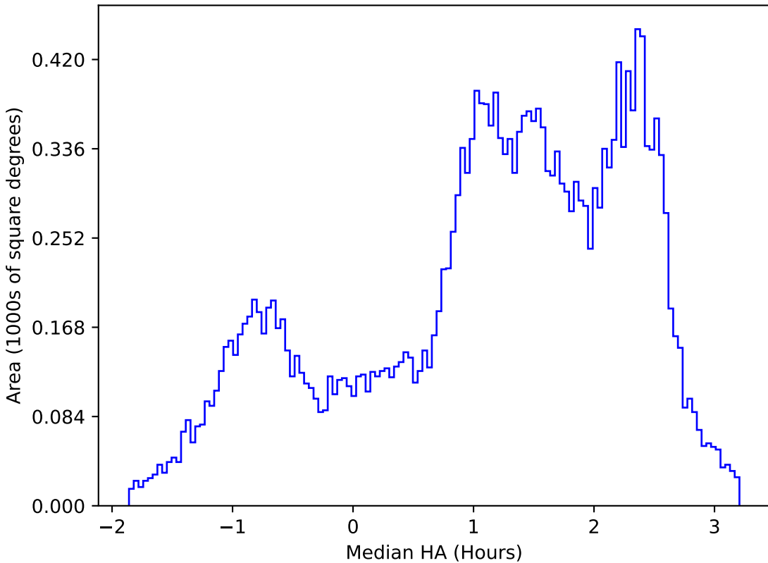
weather_cloudso18v3.4_10yrs All sky y band: Median HA
