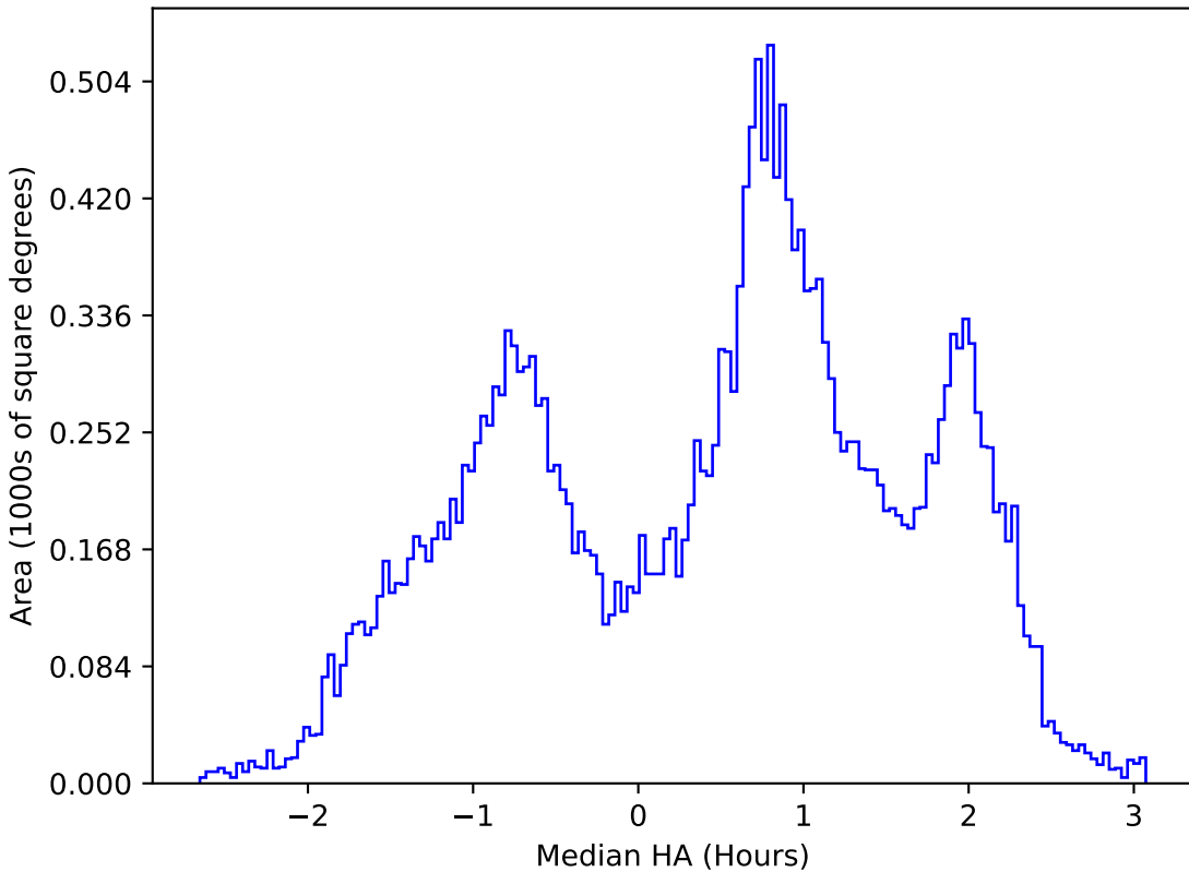
weather_cloudso18v3.4_10yrs All sky r band: Median HA
