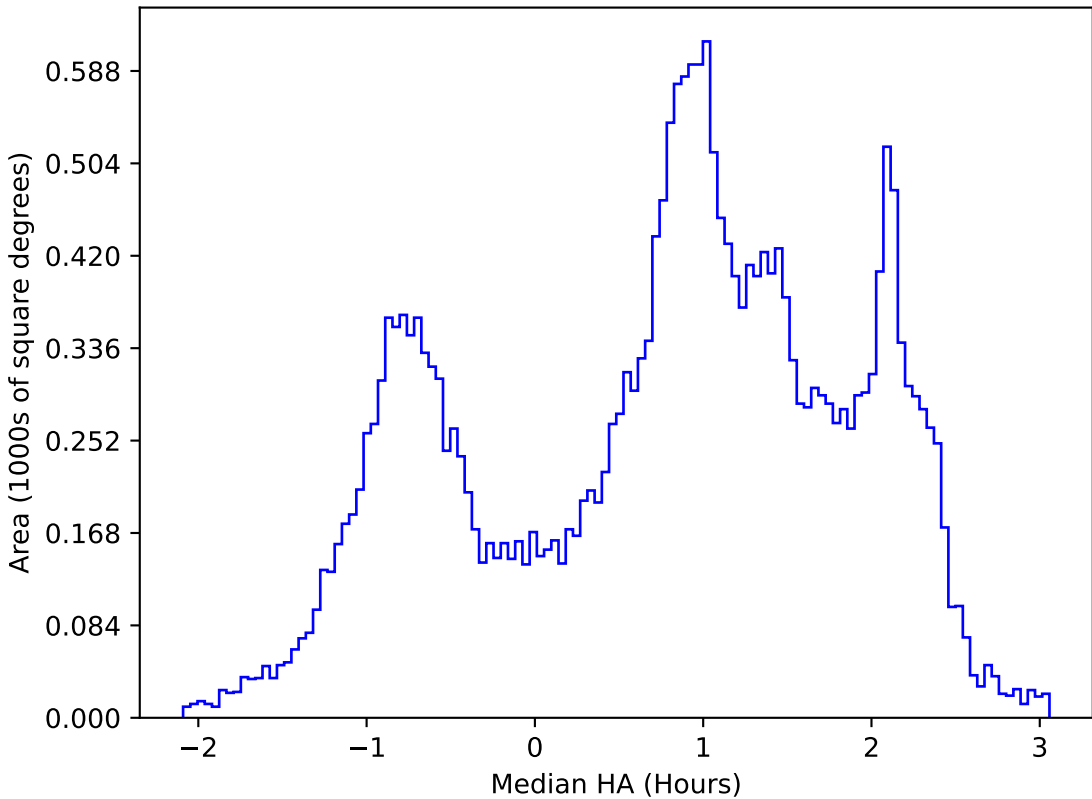
weather_cloudso18v3.4_10yrs All sky all bands: Median HA
