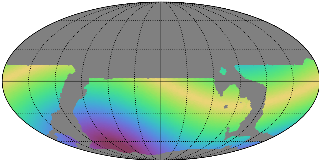
weather_cloudso18v3.4_10yrs WFD all bands: Max solarElong
