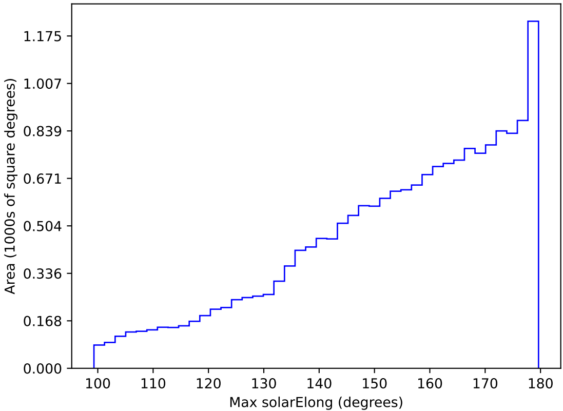
weather_cloudso18v3.4_10yrs WFD all bands: Max solarElong
