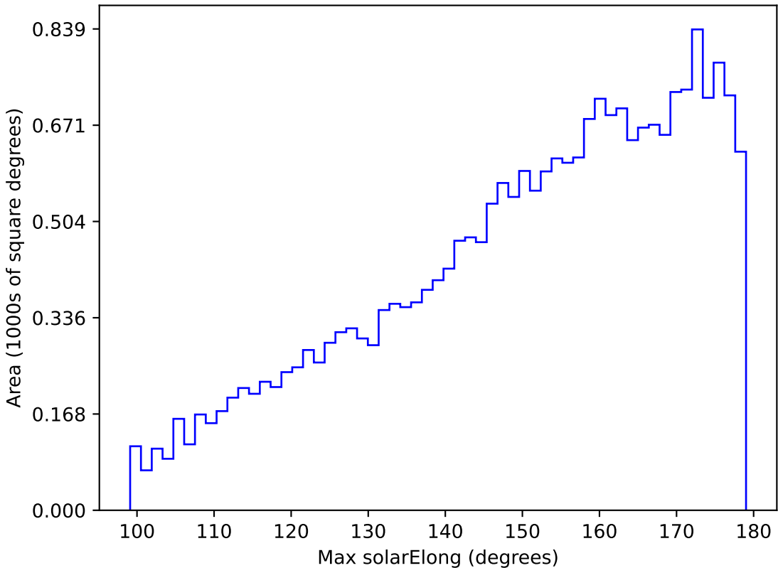
weather_cloudso18v3.4_10yrs All sky u band: Max solarElong
