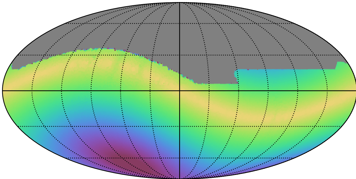
weather_cloudso18v3.4_10yrs All sky all bands: Max solarElong
