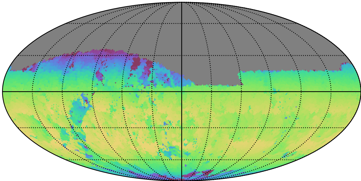
weather_cloudso18v3.4_10yrs Yr 1 z band: Max skyBrightness
