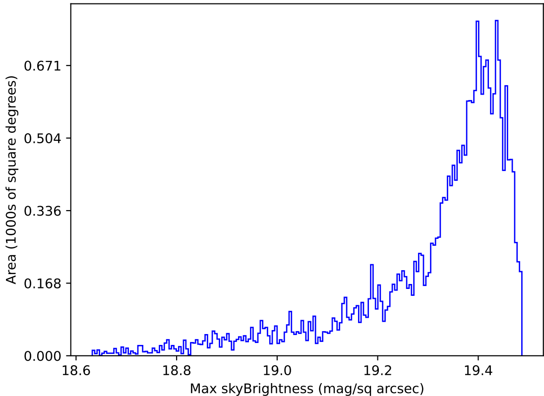
weather_cloudso18v3.4_10yrs Yr 1 z band: Max skyBrightness
