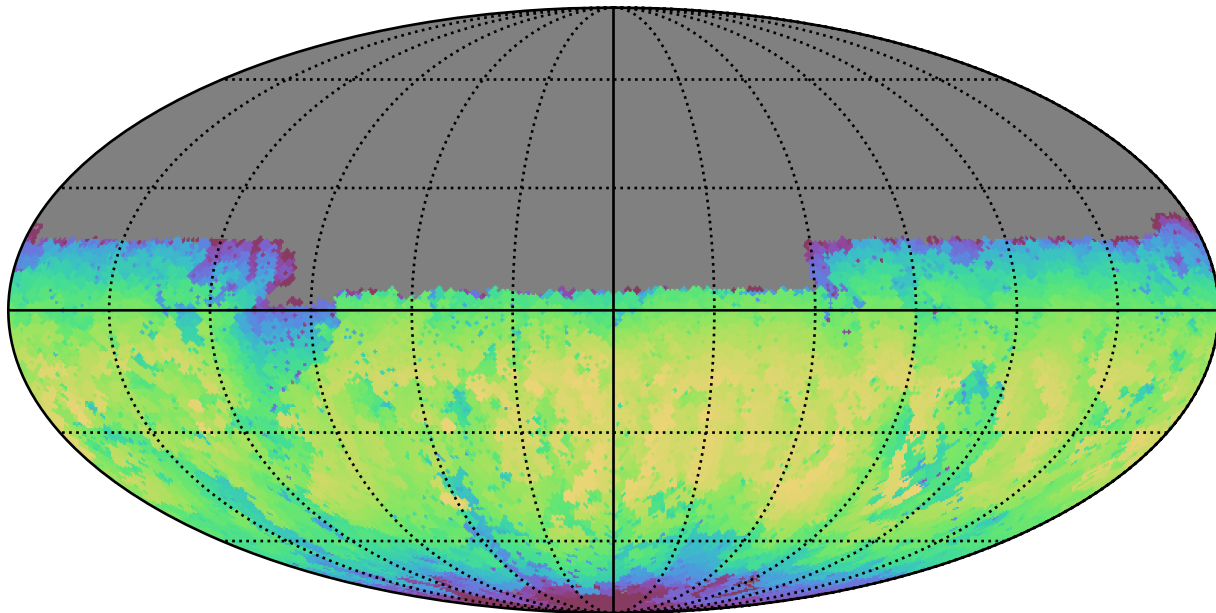
weather_cloudso18v3.4_10yrs Yr 1 y band: Max skyBrightness
