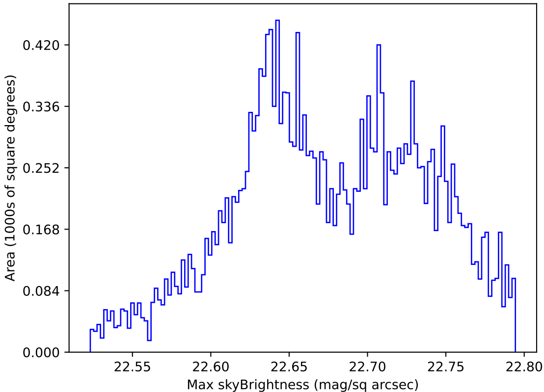
weather_cloudso18v3.4_10yrs Yr 1 u band: Max skyBrightness
