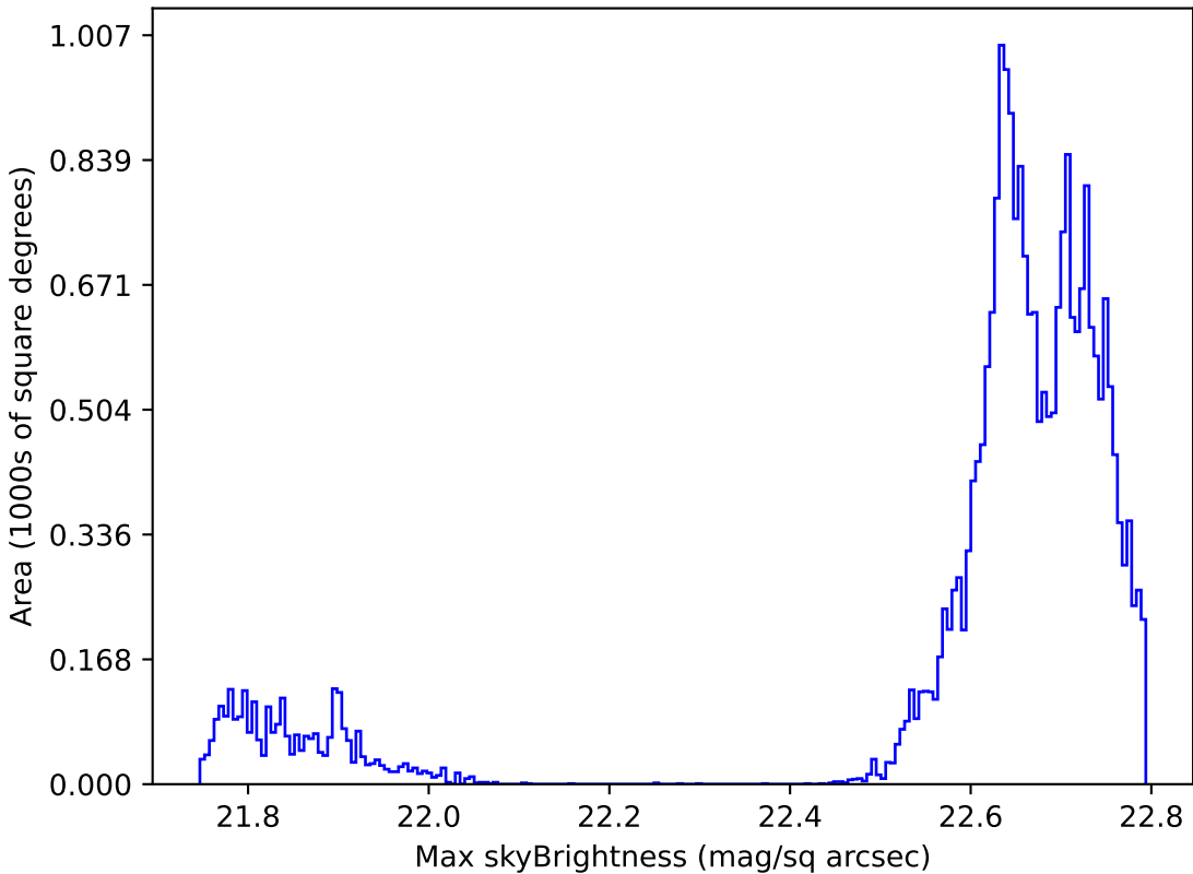
weather_cloudso18v3.4_10yrs Yr 1 all bands: Max skyBrightness
