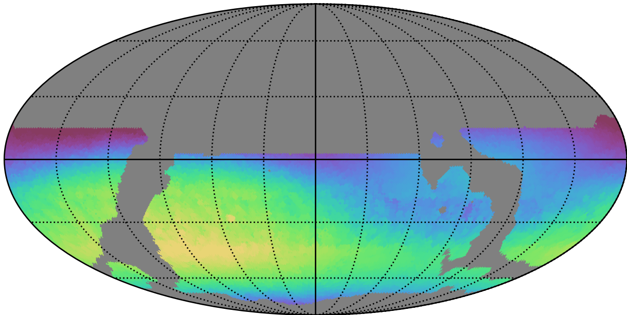
weather_cloudso18v3.4_10yrs WFD u band: Max skyBrightness
