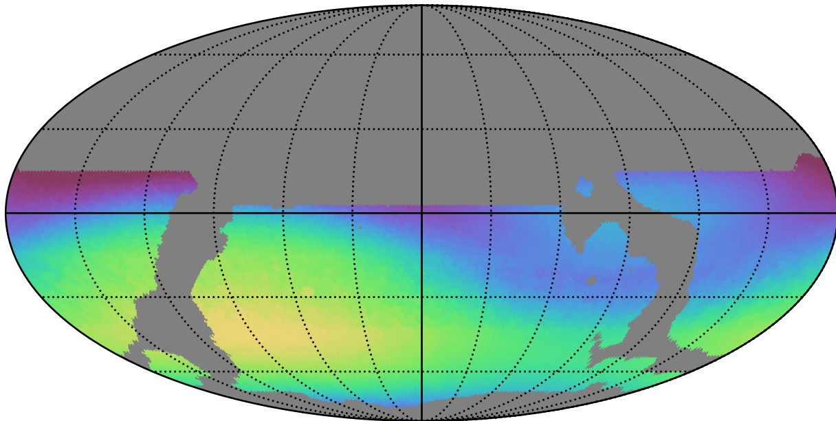
weather_cloudso18v3.4_10yrs WFD r band: Max skyBrightness
