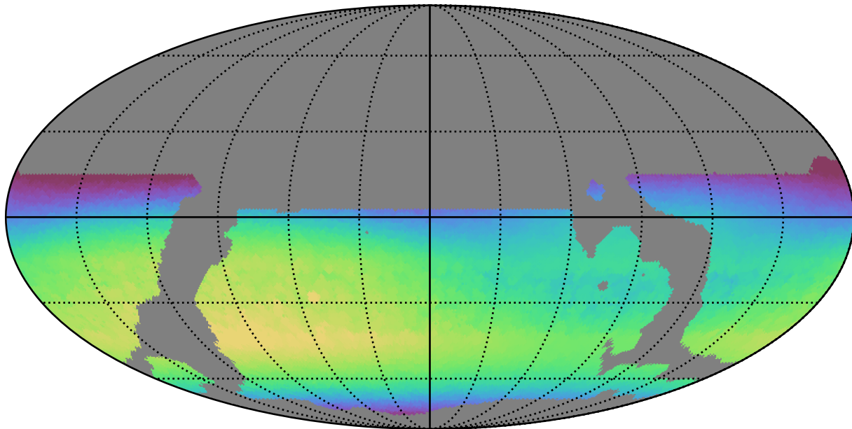
weather_cloudso18v3.4_10yrs WFD i band: Max skyBrightness
