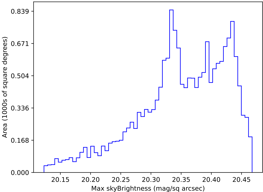
weather_cloudso18v3.4_10yrs WFD i band: Max skyBrightness
