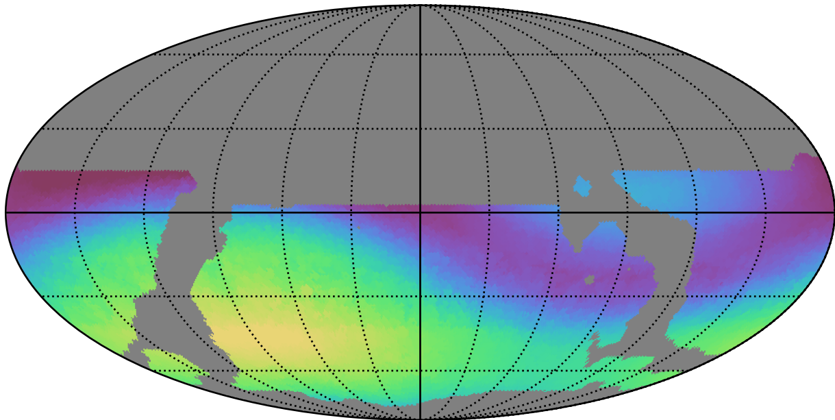
weather_cloudso18v3.4_10yrs WFD g band: Max skyBrightness
