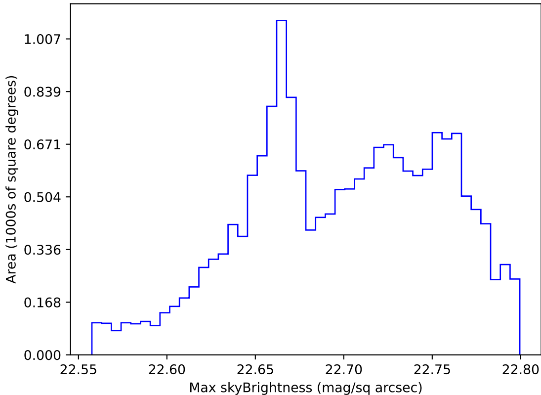
weather_cloudso18v3.4_10yrs WFD all bands: Max skyBrightness
