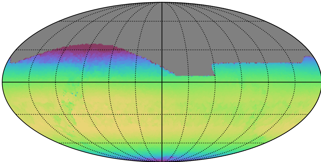
weather_cloudso18v3.4_10yrs All sky z band: Max skyBrightness
