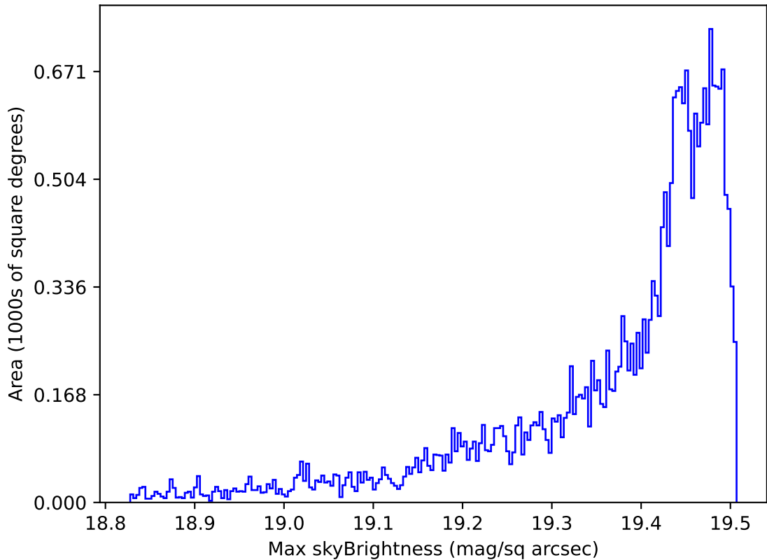
weather_cloudso18v3.4_10yrs All sky z band: Max skyBrightness
