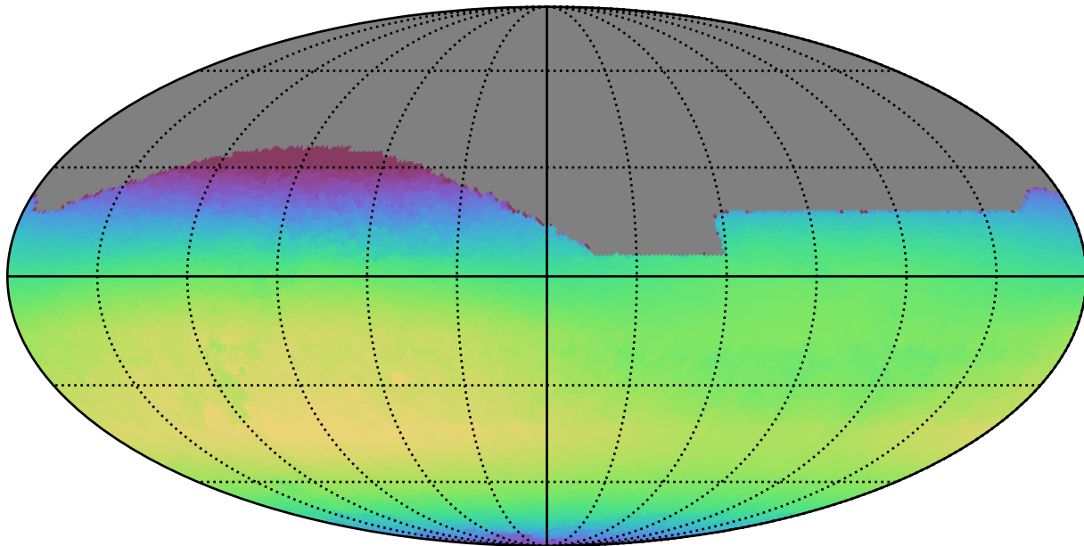
weather_cloudso18v3.4_10yrs All sky i band: Max skyBrightness
