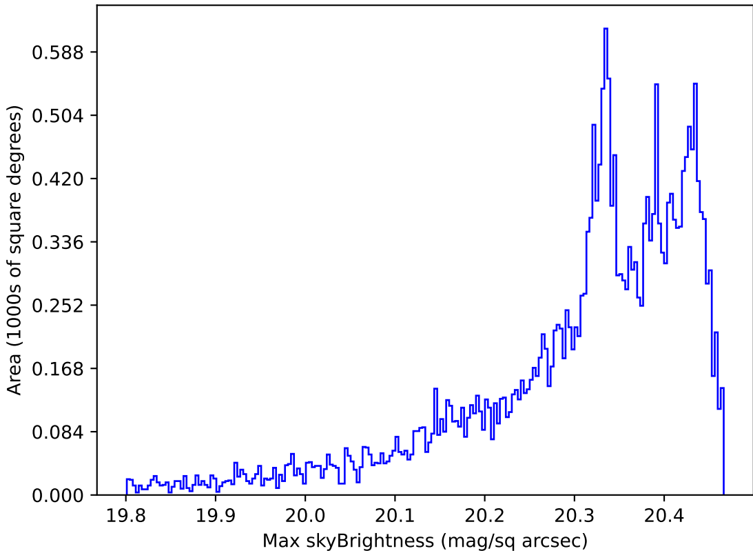
weather_cloudso18v3.4_10yrs All sky i band: Max skyBrightness
