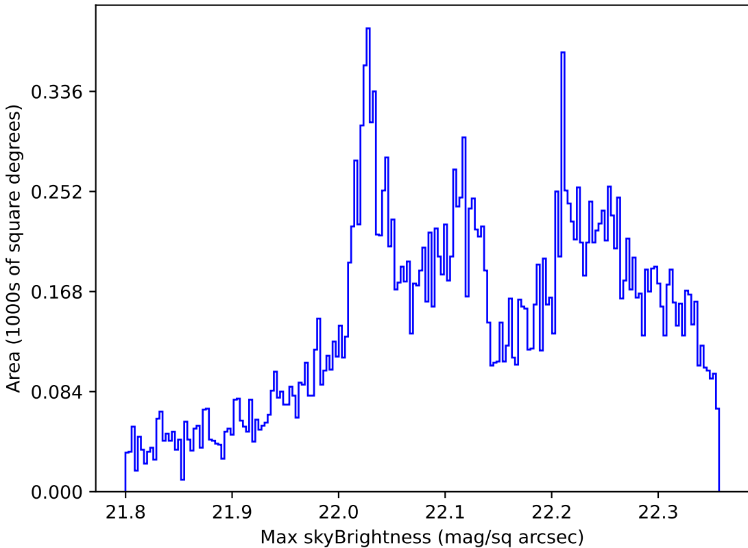
weather_cloudso18v3.4_10yrs All sky g band: Max skyBrightness
