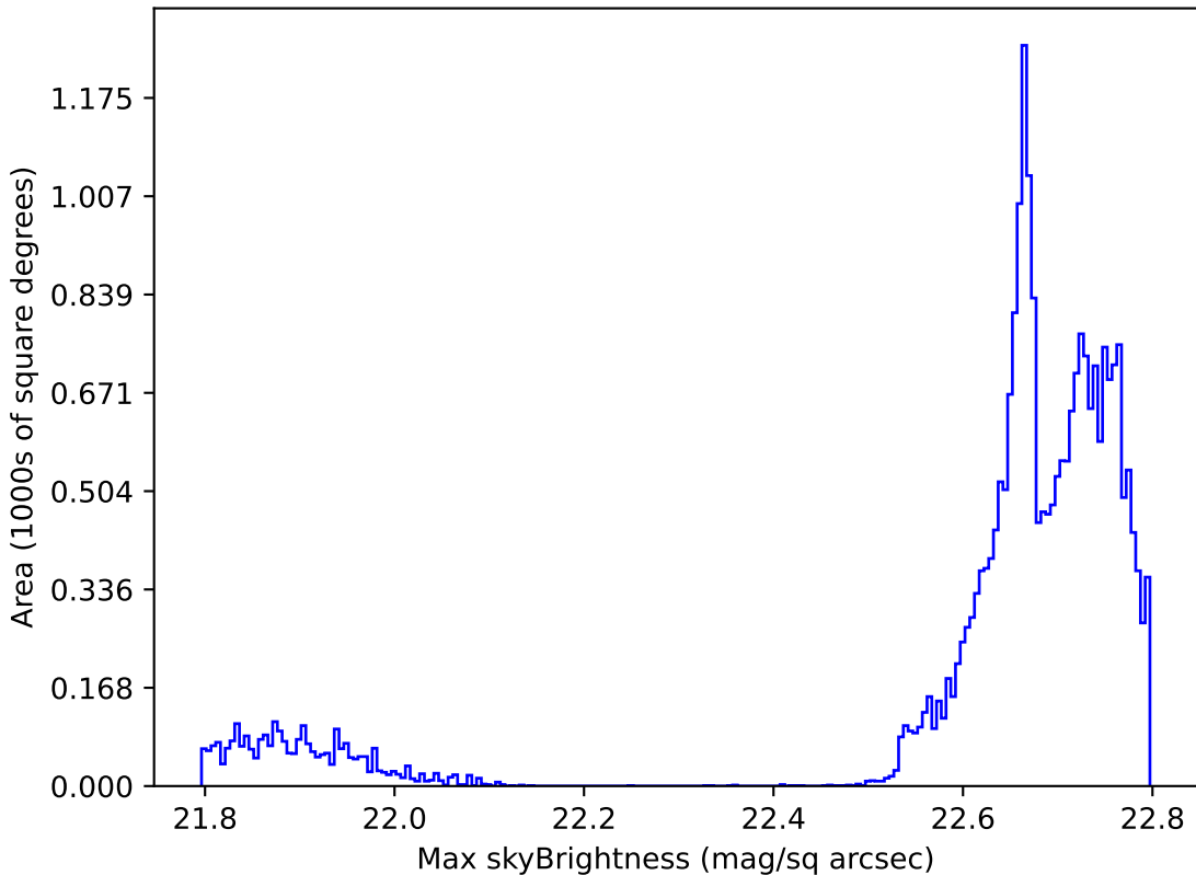
weather_cloudso18v3.4_10yrs All sky all bands: Max skyBrightness
