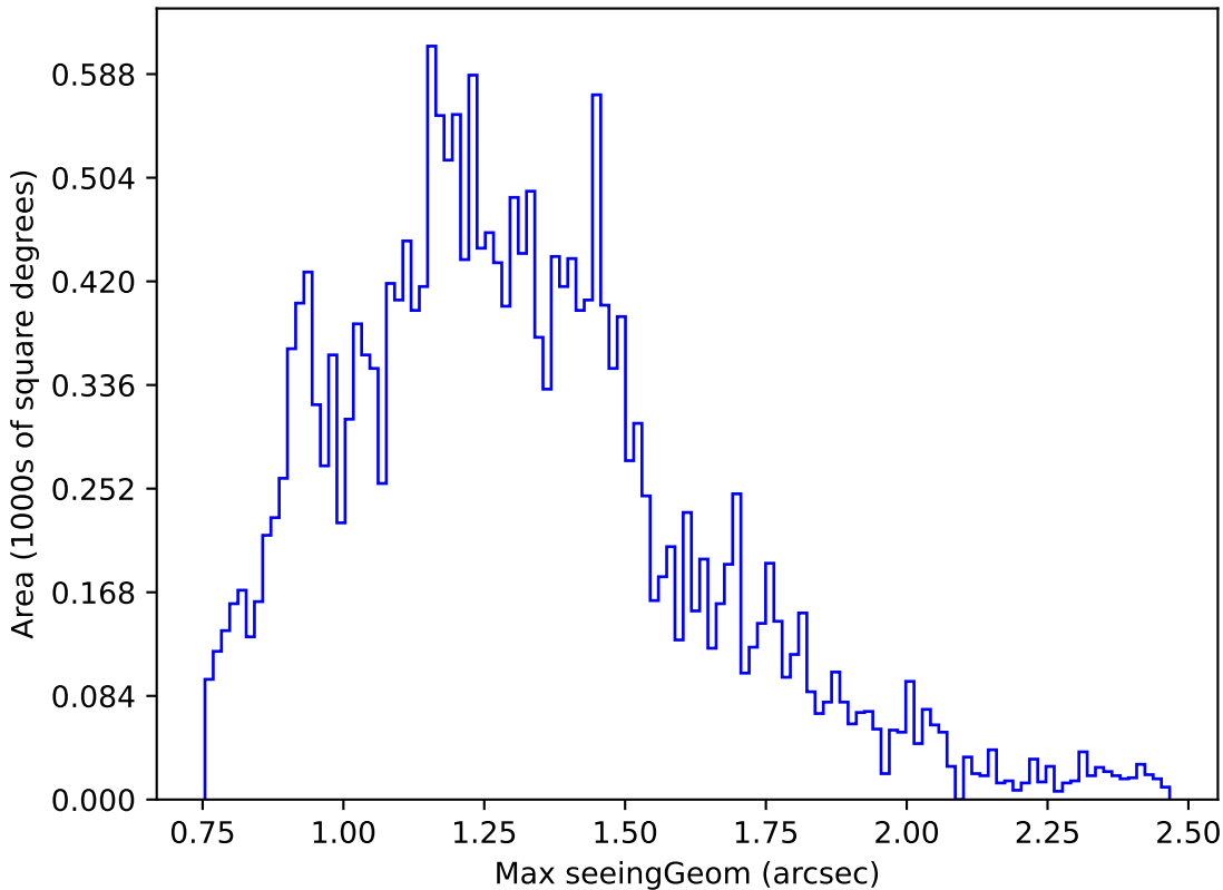
weather_cloudso18v3.4_10yrs Yr 1 u band: Max seeingGeom
