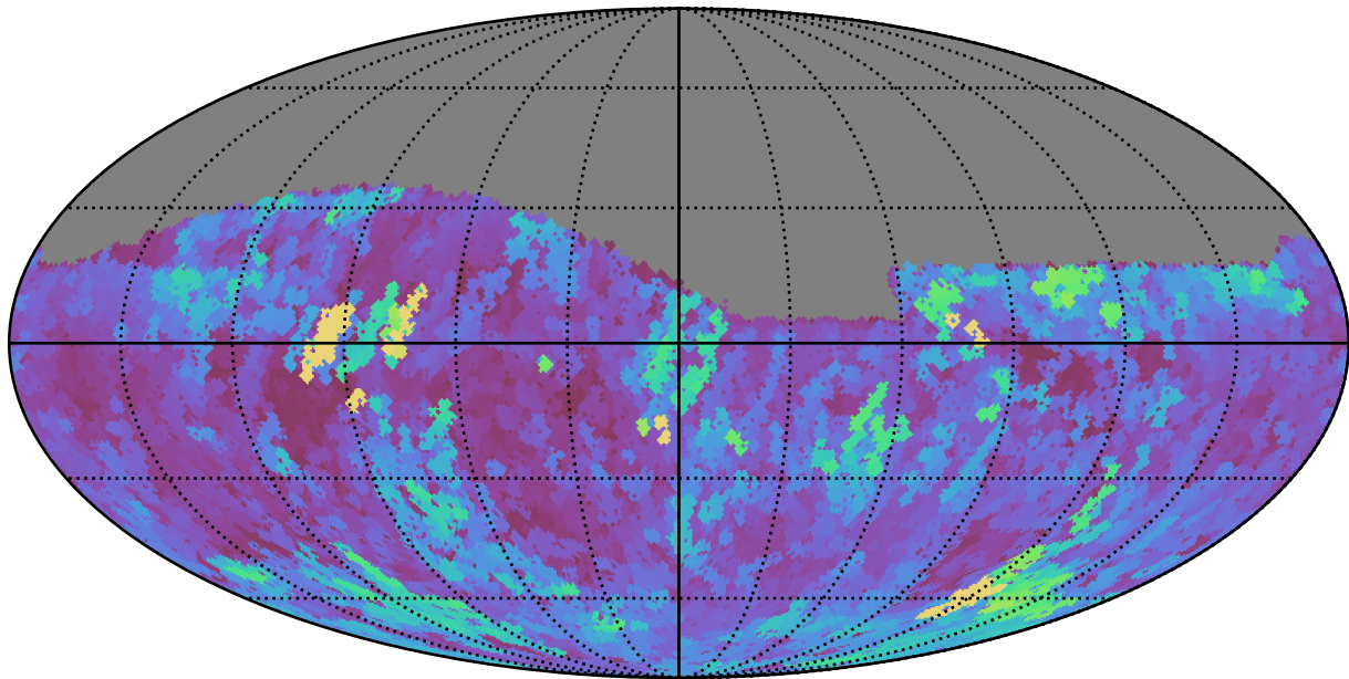
weather_cloudso18v3.4_10yrs Yr 1 r band: Max seeingGeom
