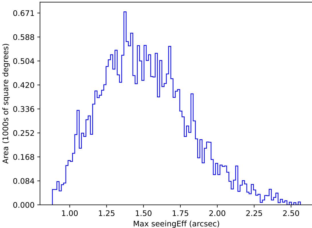
weather_cloudso18v3.4_10yrs Yr 1 z band: Max seeingEff
