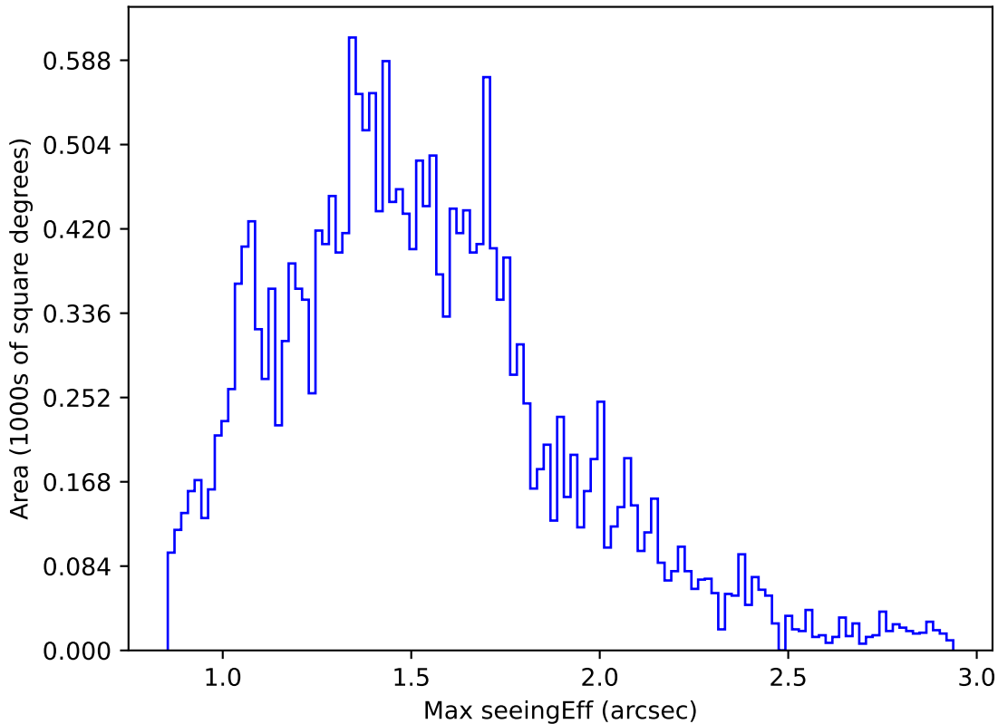
weather_cloudso18v3.4_10yrs Yr 1 u band: Max seeingEff
