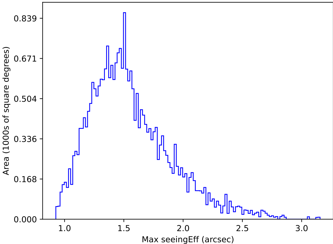
weather_cloudso18v3.4_10yrs Yr 1 r band: Max seeingEff
