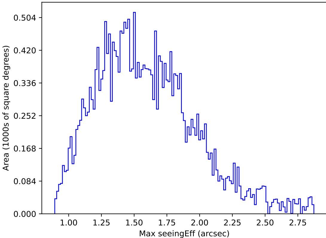
weather_cloudso18v3.4_10yrs Yr 1 i band: Max seeingEff
