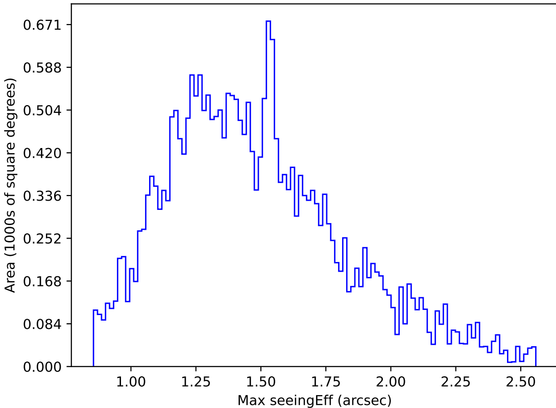
weather_cloudso18v3.4_10yrs Yr 1 g band: Max seeingEff
