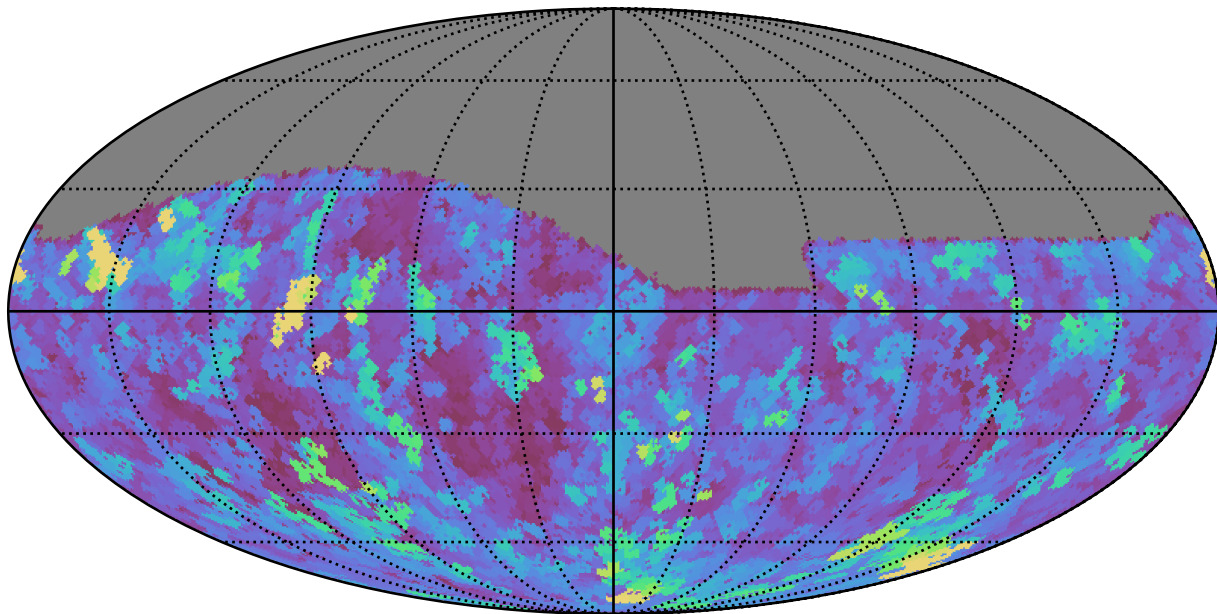
weather_cloudso18v3.4_10yrs Yr 1 all bands: Max seeingEff
