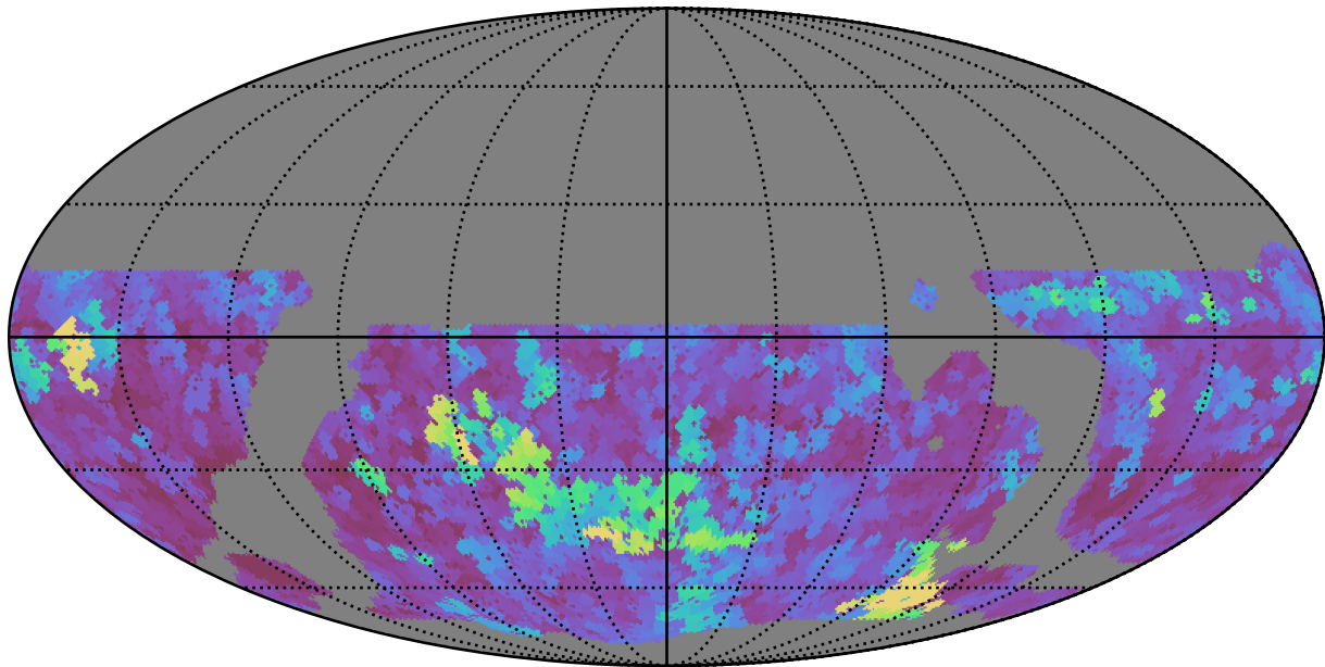
weather_cloudso18v3.4_10yrs WFD z band: Max seeingEff
